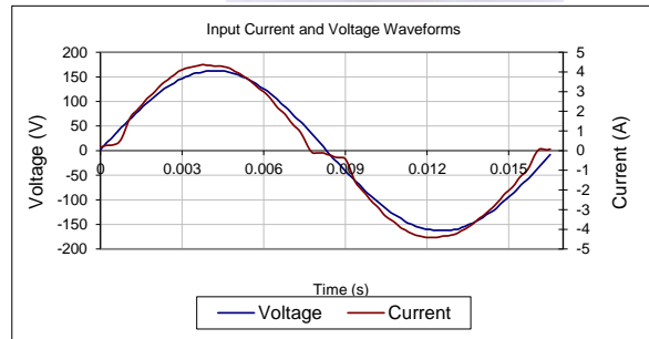
Input AC Current Waveform (ITHD = 10.18%, 50% Load)
